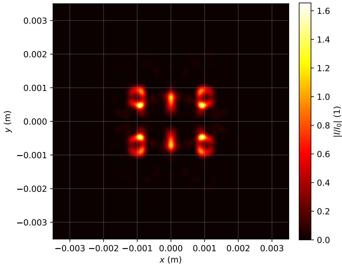
Intensity profile I(x, y, z = 1.353)/I_0 , P_{in}=13.0\text{Pcr} , artificial time
