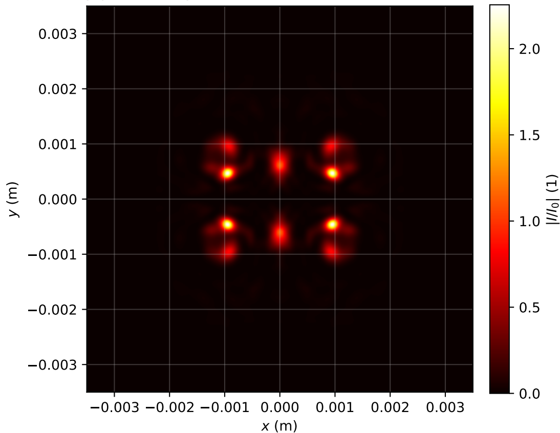
Intensity profile I(x, y, z = 1.433)/I_0 , P_{in}=13.0\text{Pcr} , artificial time
