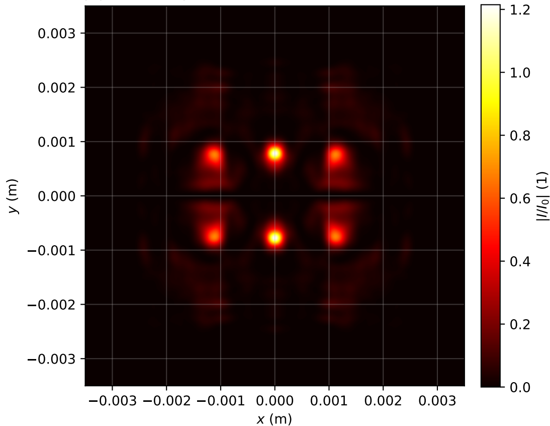
Intensity profile I(x, y, z = 2.388)/I_0 , P_{in}=13.0\text{Pcr} , artificial time
