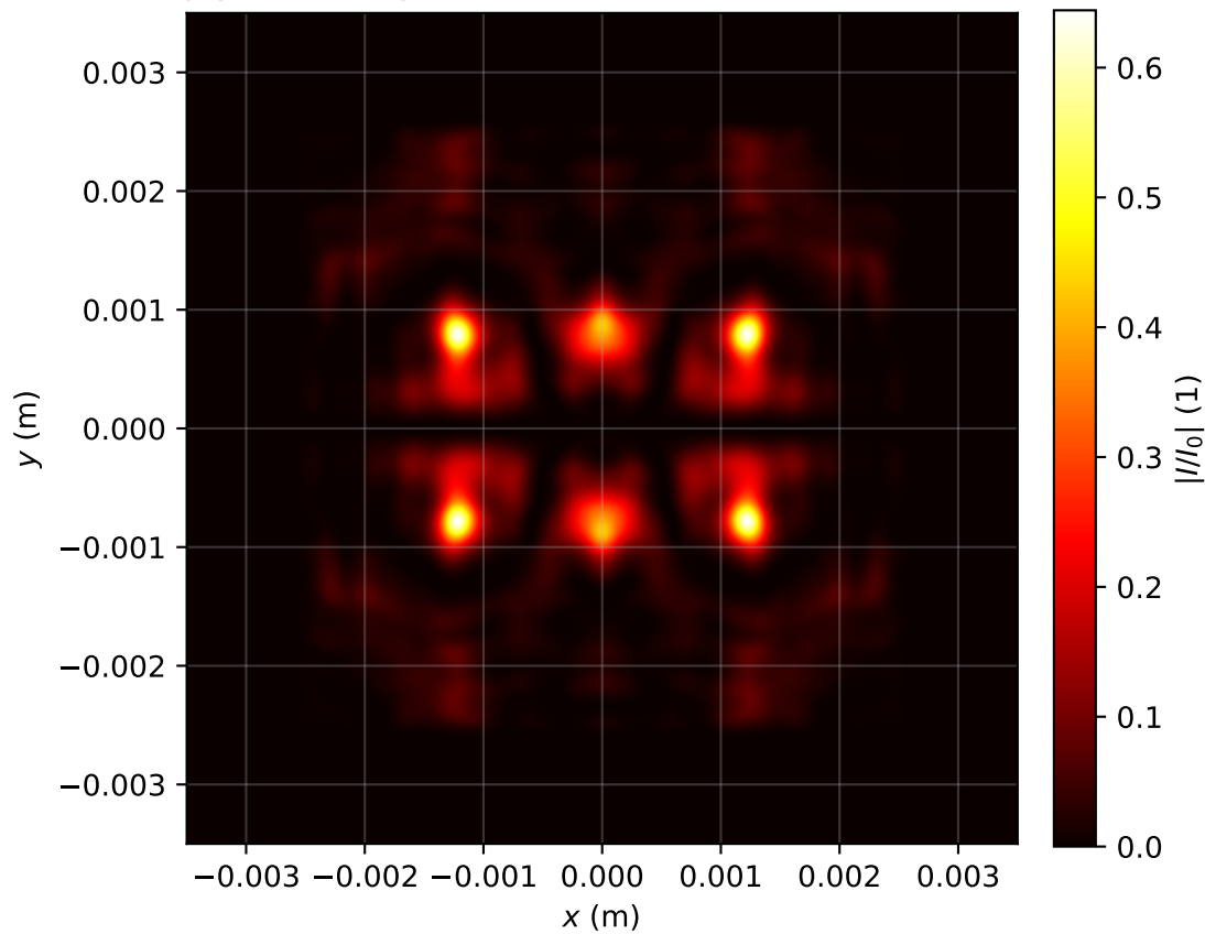
Intensity profile I(x, y, z = 2.627)/I_0 , P_{in}=13.0P_{cr} , artificial time
