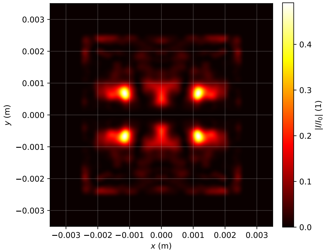
Intensity profile I(x, y, z = 3.344)/I_0 , P_{in}=13.0\text{Pcr} , artificial time
