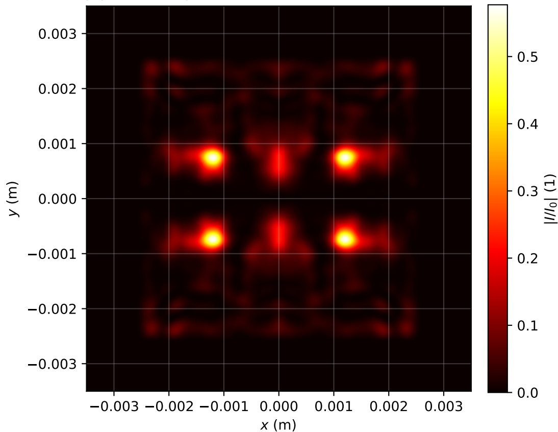
Intensity profile I(x, y, z = 3.503)/I_0 , P_{in}=13.0P_{cr} , artificial time
