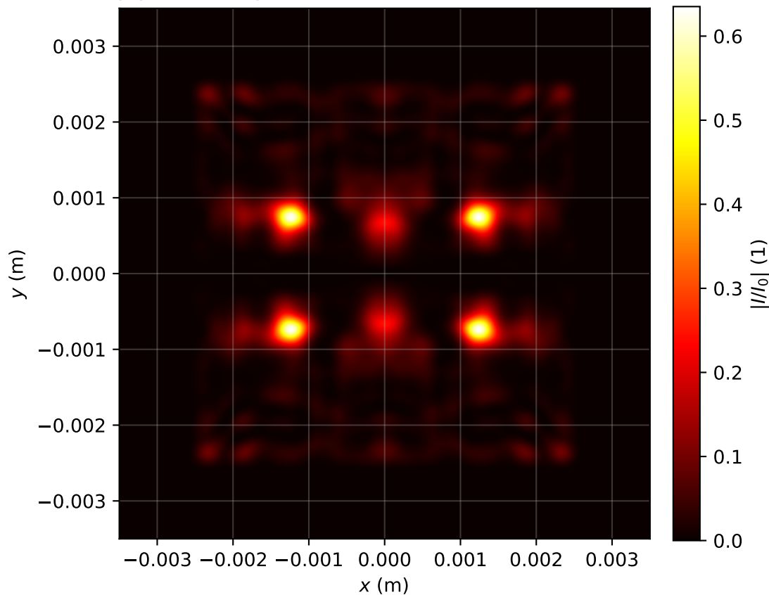
Intensity profile I(x, y, z = 3.582)/I_0 , P_{in}=13.0P_{cr} , artificial time
