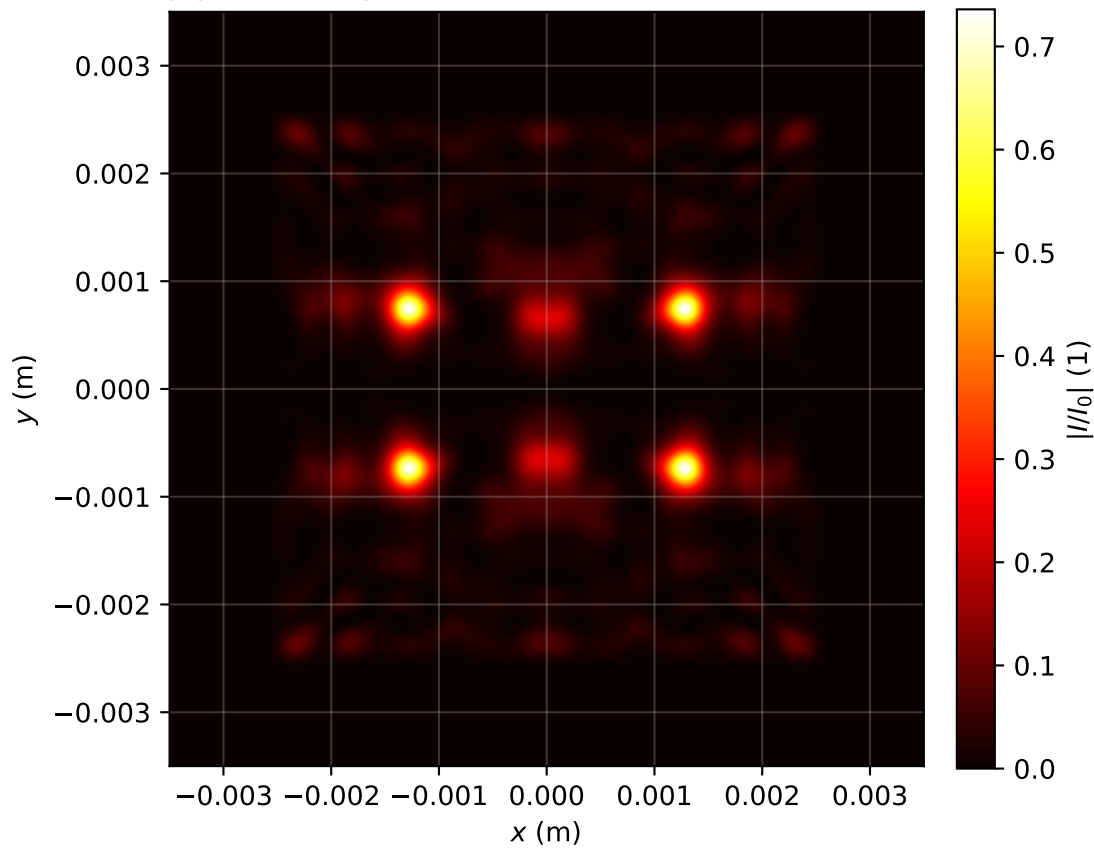
Intensity profile I(x, y, z = 3.662)/I_0 , P_{in}=13.0P_{cr} , artificial time
