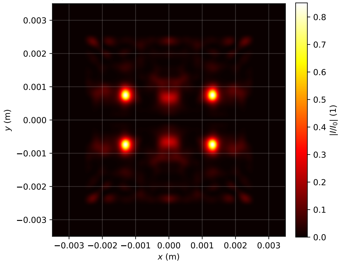
Intensity profile I(x, y, z = 3.742)/I_0 , P_{in}=13.0P_{cr} , artificial time
