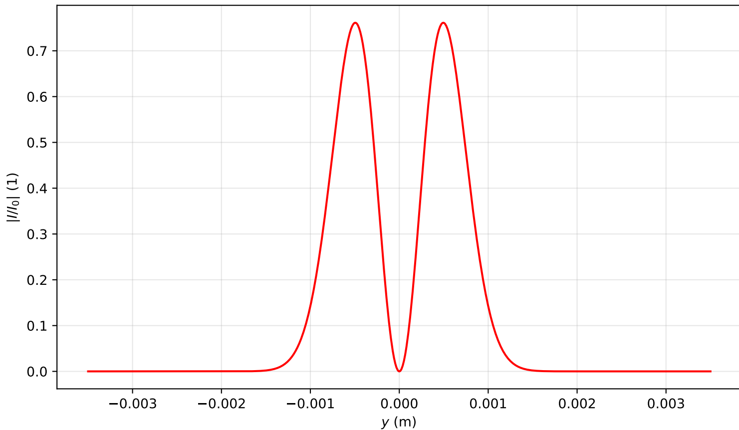
Intensity profile I(x=0, y, z=0.000)/I_0 , P_{in}=13.0P_{cr} , artificial time
