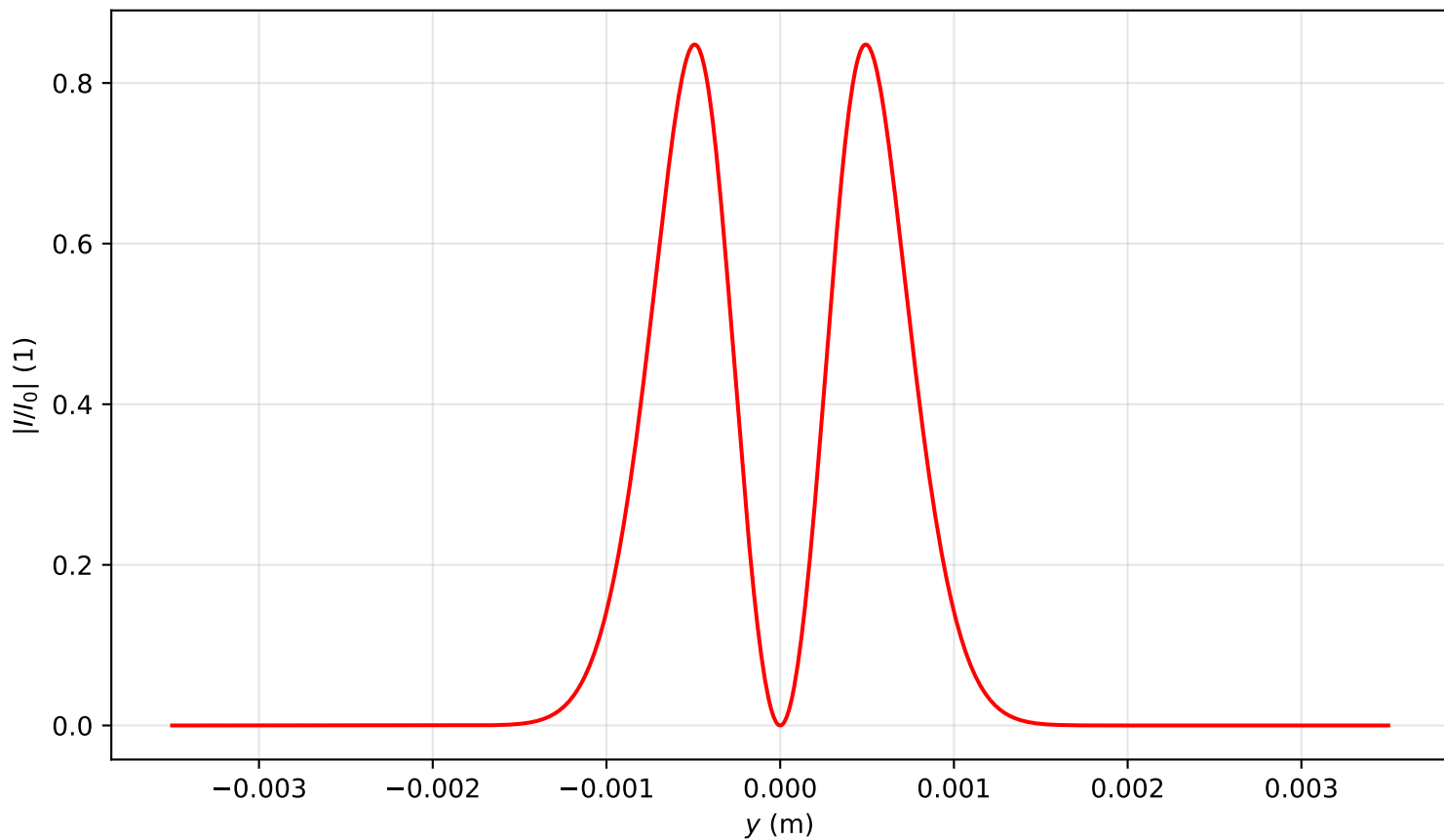
Intensity profile I(x=0, y, z=0.080)/I_0 , P_{in}=13.0P_{cr} , artificial time
