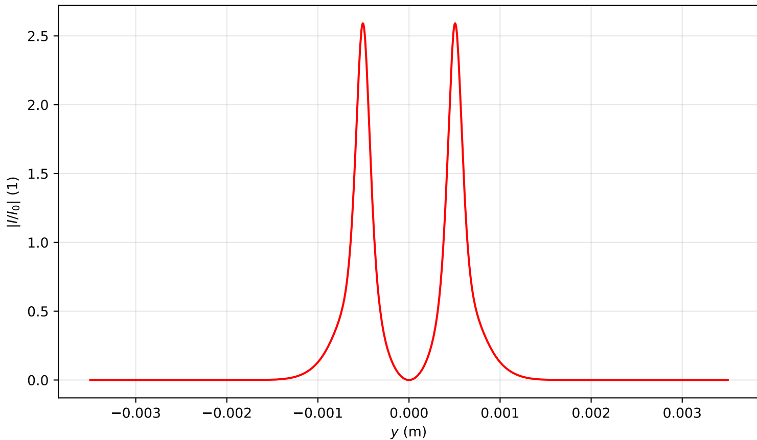
Intensity profile I(x=0, y, z=0.318)/I_0 , P_{in}=13.0P_{cr} , artificial time
