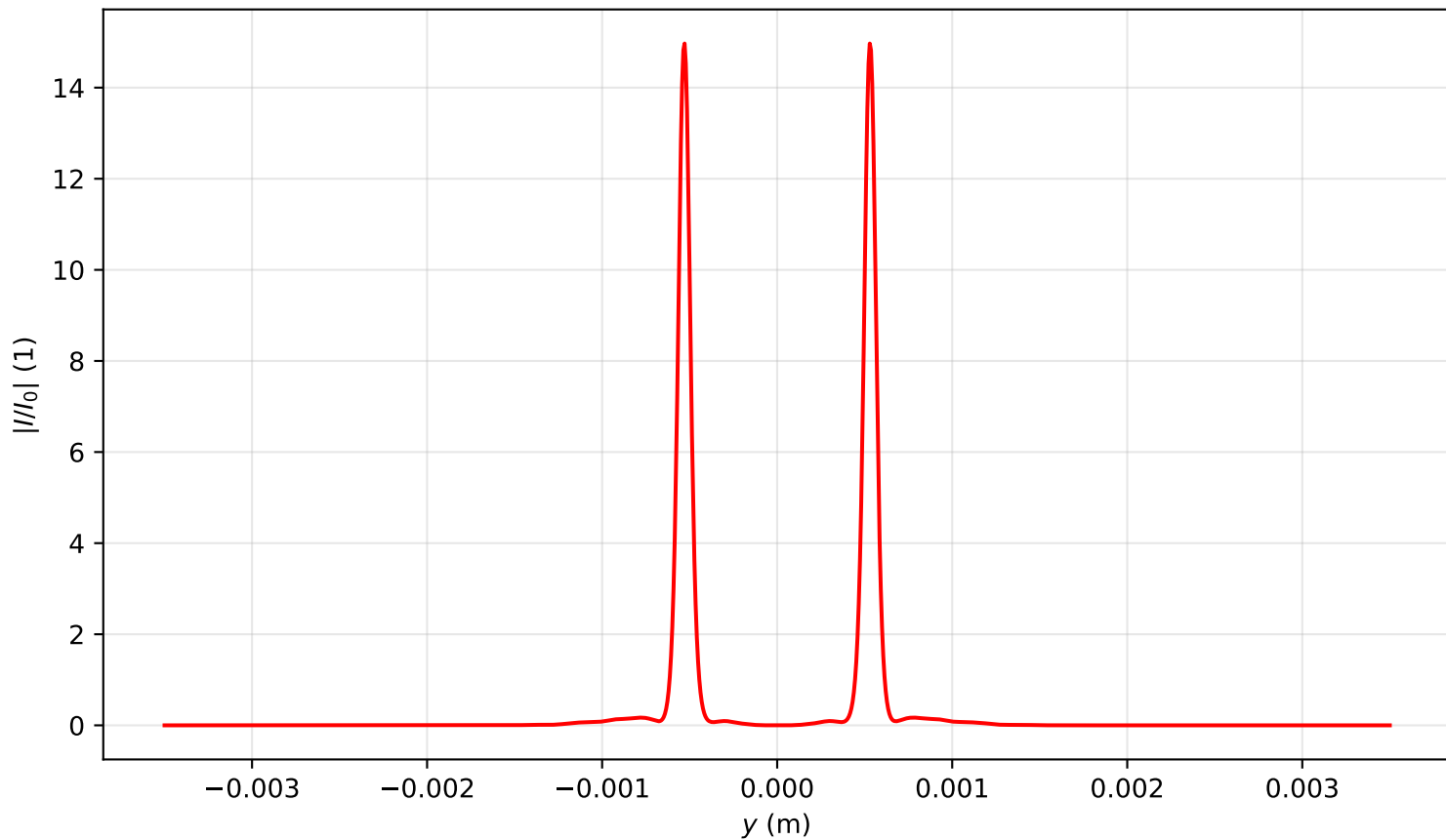
Intensity profile I(x=0, y, z=0.557)/I_0 , \text{Pin}=13.0\text{Pcr} , artificial time
