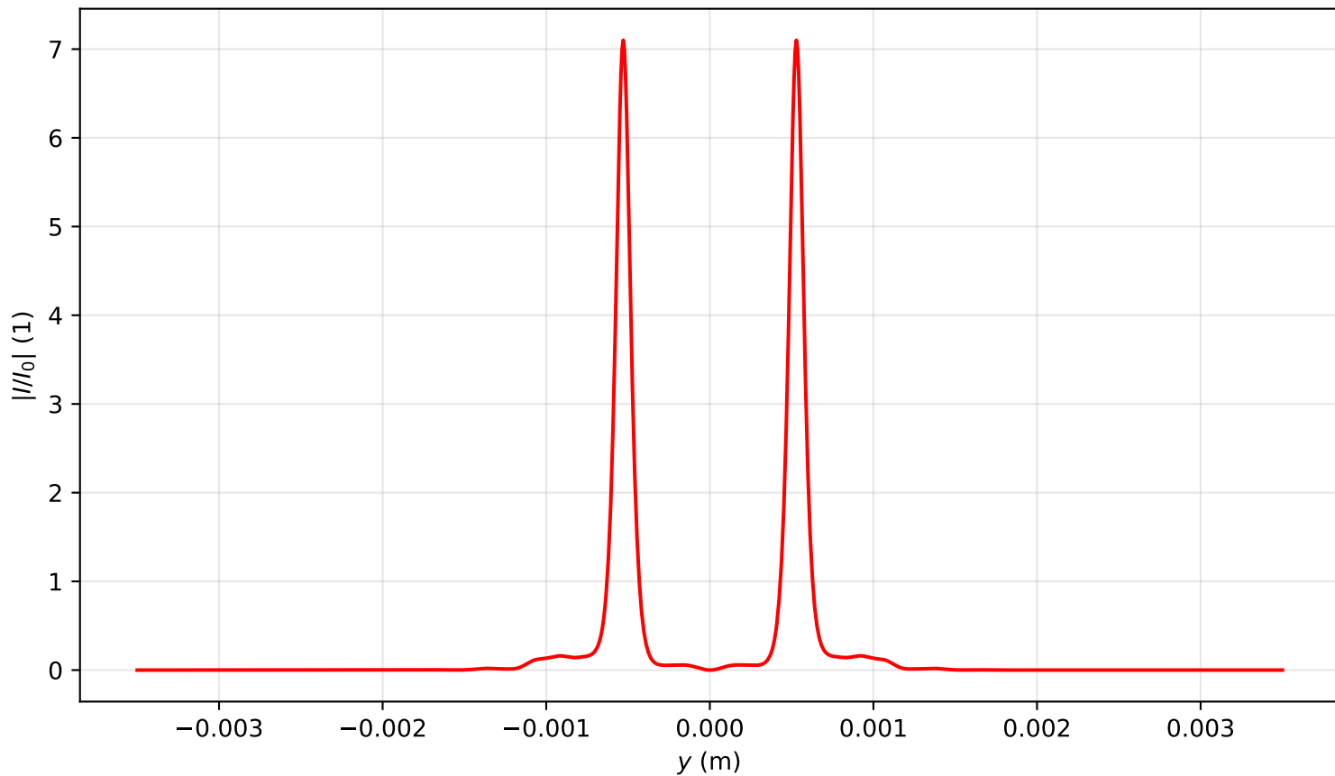
Intensity profile I(x=0, y, z=0.637)/I_0 , \text{Pin}=13.0\text{Pcr} , artificial time
