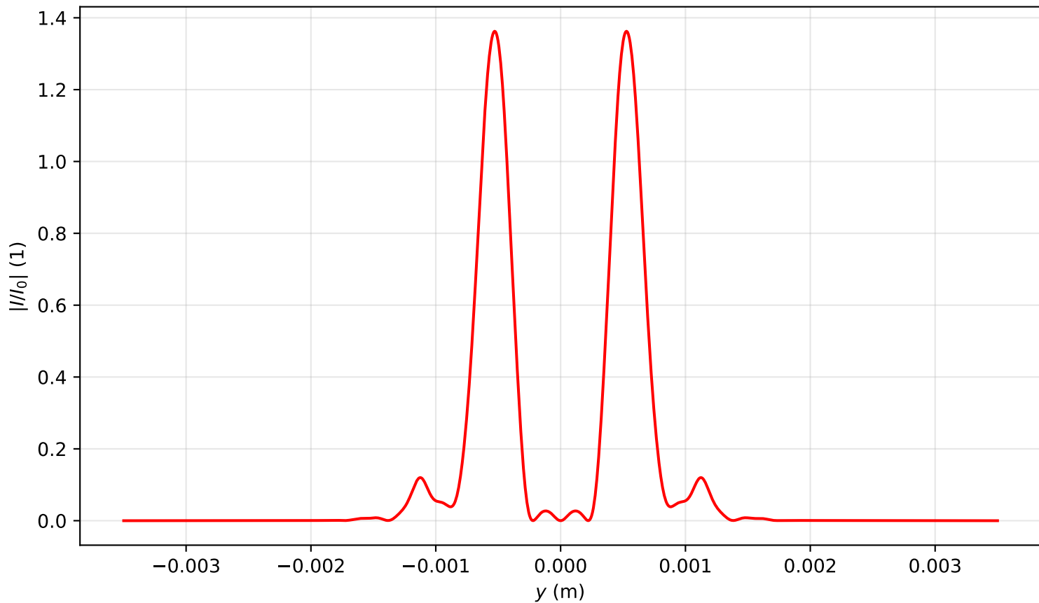
Intensity profile I(x=0, y, z=0.716)/I_0 , P_{in}=13.0P_{cr} , artificial time
