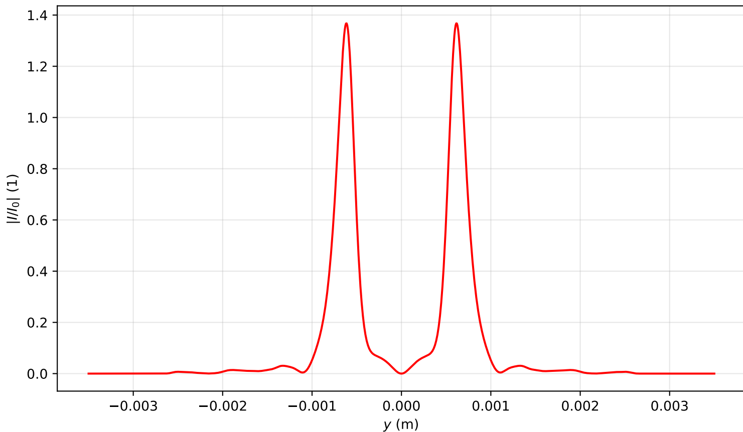
Intensity profile I(x=0, y, z=1.513)/I_0 , P_{in}=13.0P_{cr} , artificial time
