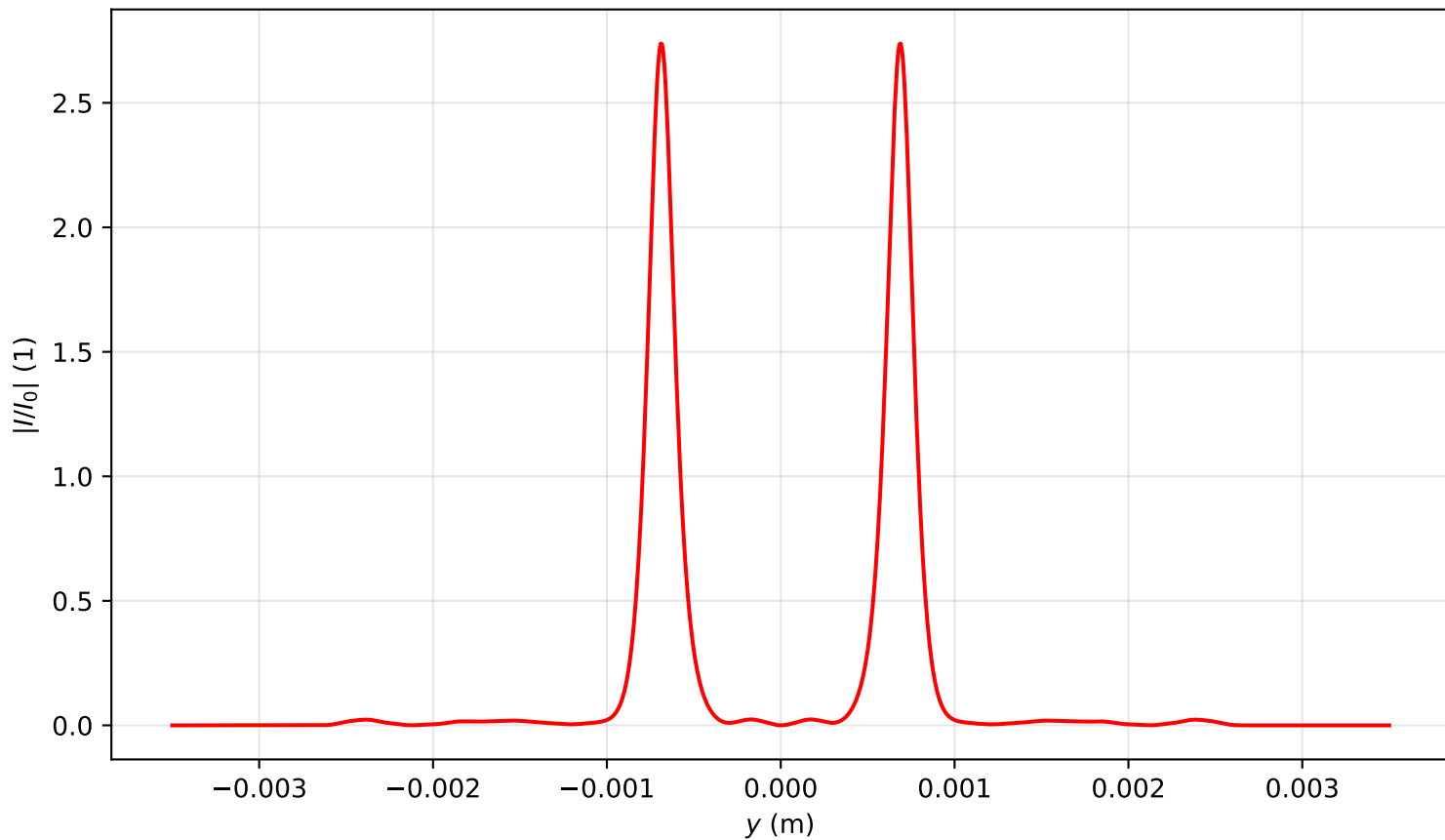
Intensity profile I(x=0, y, z=1.831)/I_0 , P_{in}=13.0P_{cr} , artificial time
