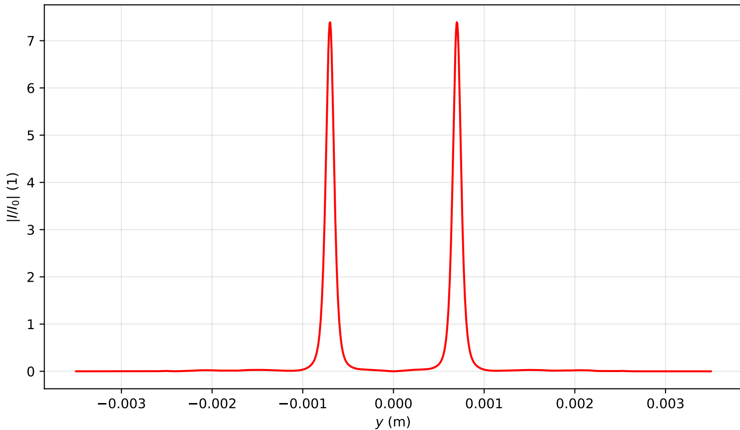
Intensity profile I(x=0, y, z=1.990)/I_0 , P_{in}=13.0\text{Pcr} , artificial time
