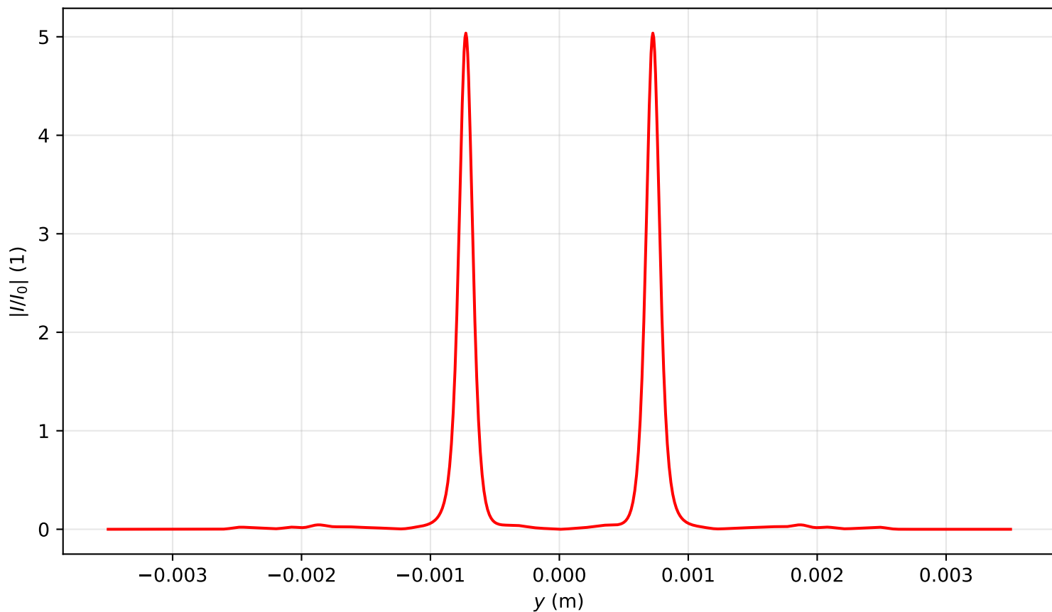
Intensity profile I(x=0, y, z=2.229)/I_0 , P_{in}=13.0\text{Pcr} , artificial time
