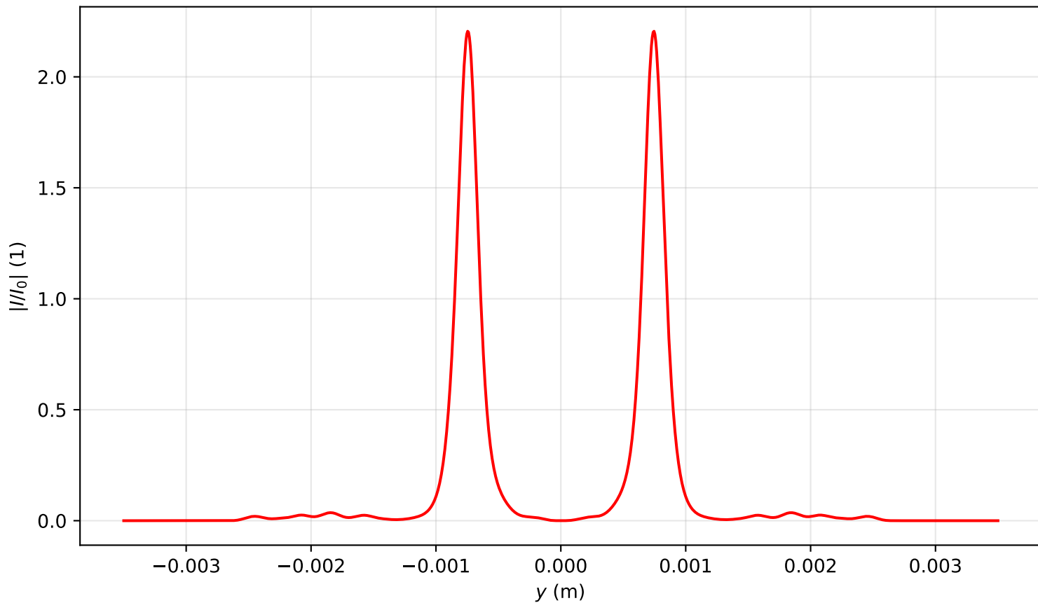
Intensity profile I(x=0, y, z=2.309)/I_0 , P_{in}=13.0P_{cr} , artificial time
