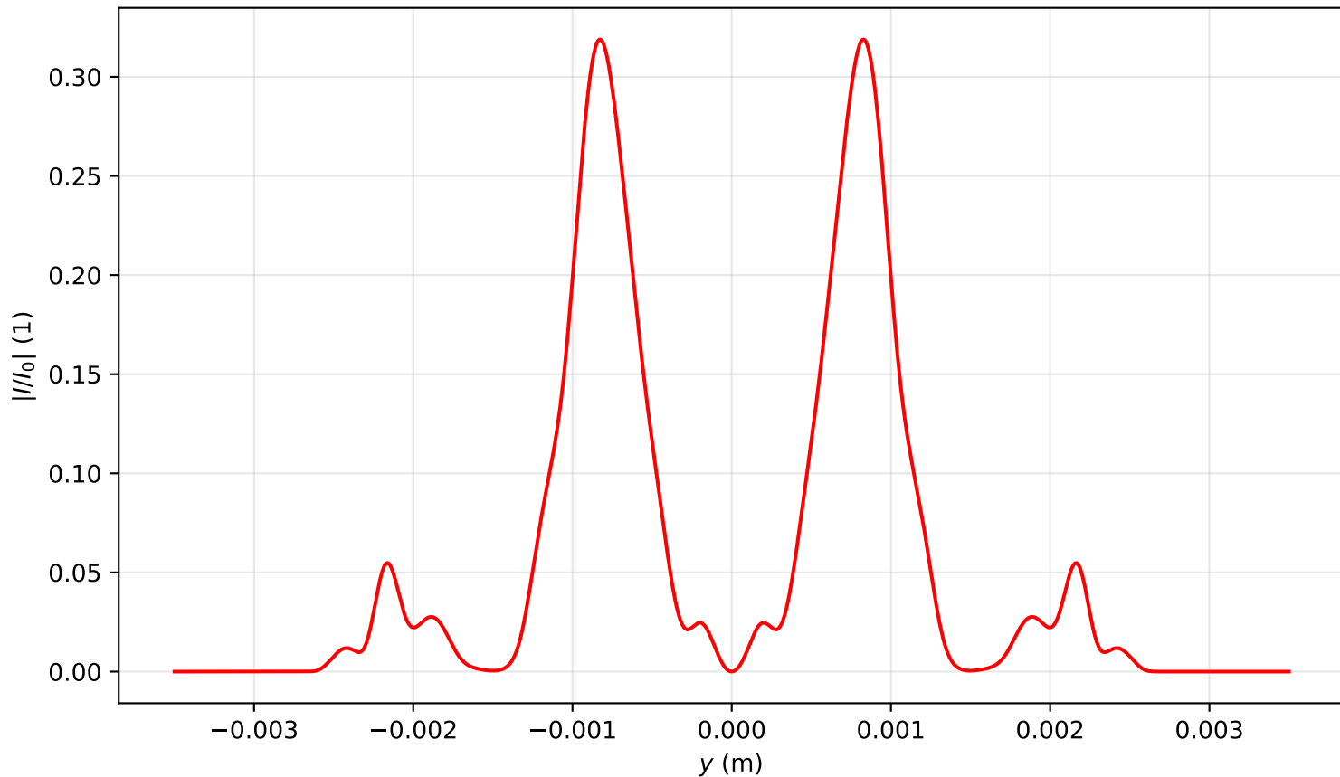
Intensity profile I(x=0, y, z=2.707)/I_0 , P_{in}=13.0P_{cr} , artificial time
