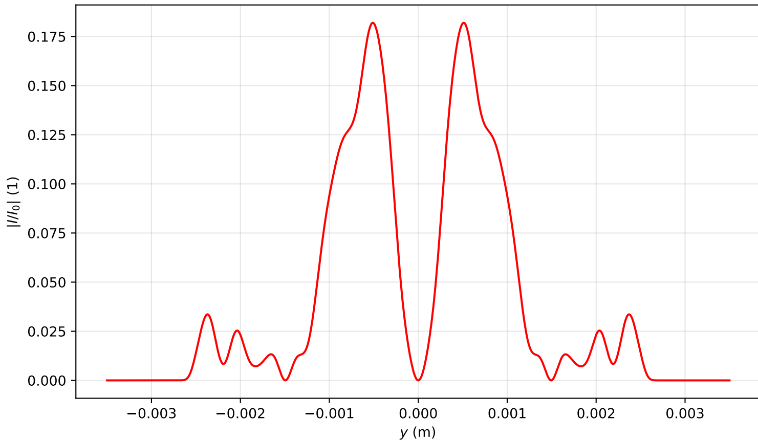
Intensity profile I(x=0, y, z=3.184)/I_0 , P_{in}=13.0P_{cr} , artificial time
