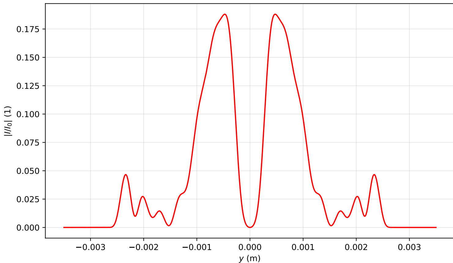
Intensity profile I(x=0, y, z=3.264)/I_0 , P_{in}=13.0\text{Pcr} , artificial time
