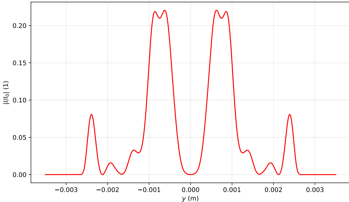
Intensity profile I(x=0, y, z=3.981)/I_0 , P_{in}=13.0P_{cr} , artificial time
