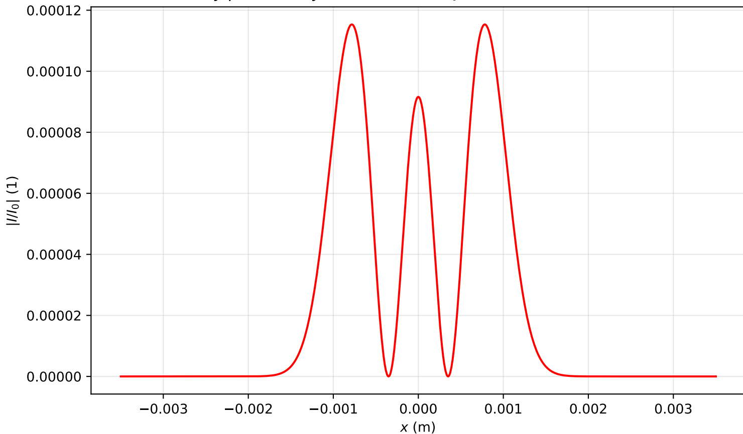
Intensity profile I(x, y = 0, z = 0.080)/I_0 , P_{in}=14.0P_{cr} , artificial time
