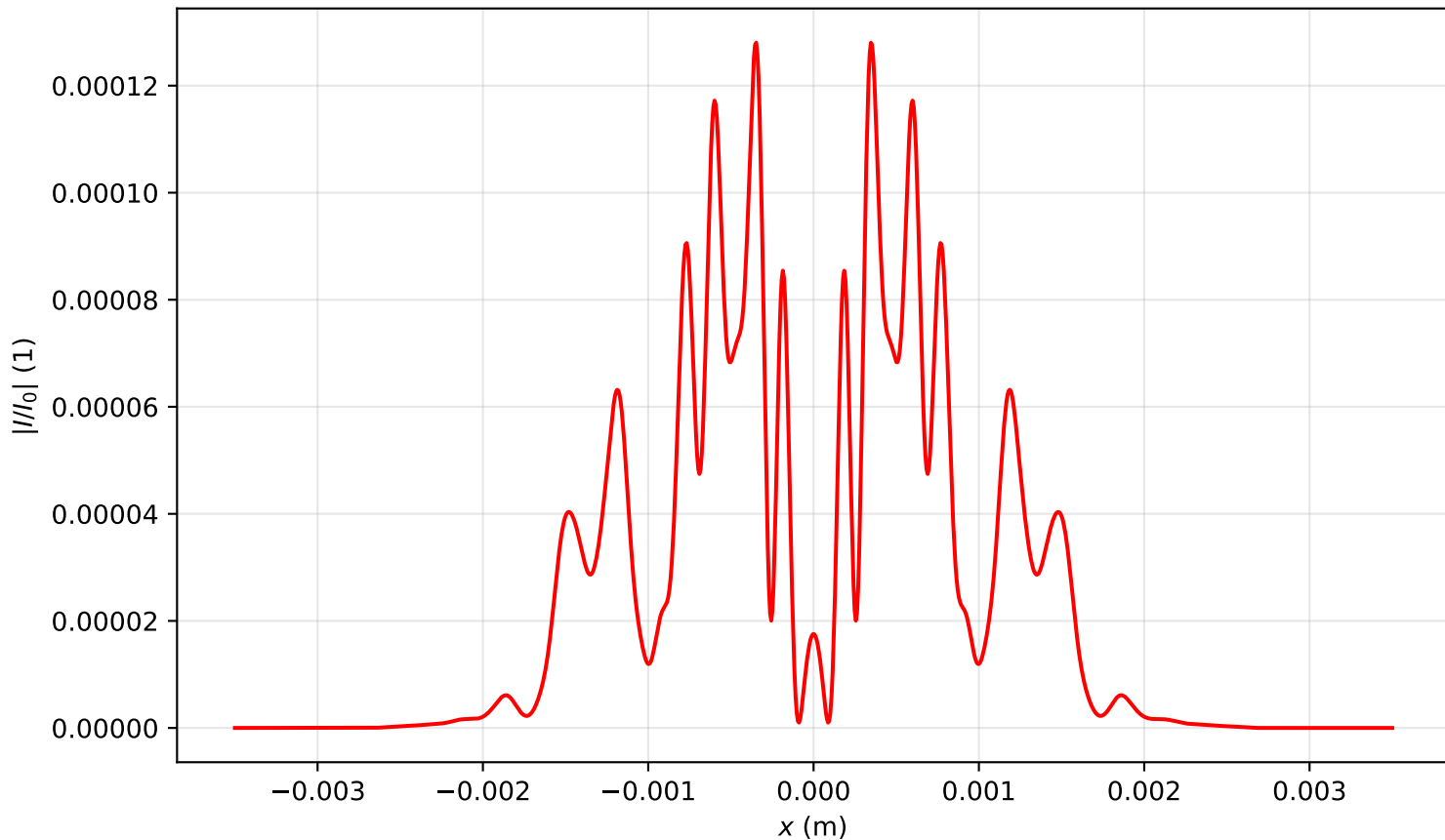
Intensity profile I(x, y = 0, z = 0.637)/I_0 , P_{in}=14.0P_{cr} , artificial time
