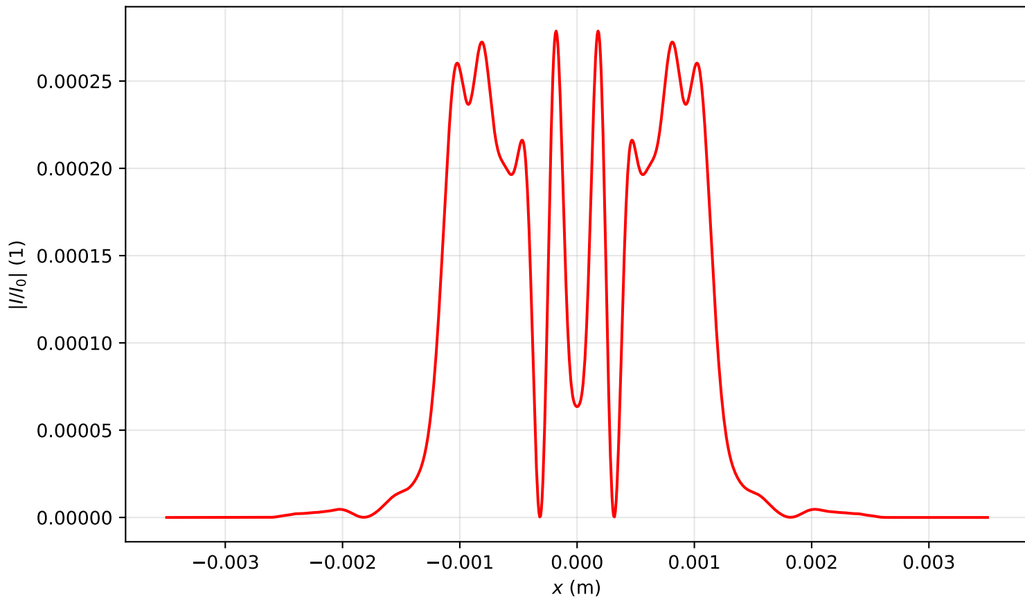
Intensity profile I(x, y = 0, z = 0.876)/I_0 , P_{in}=14.0P_{cr} , artificial time
