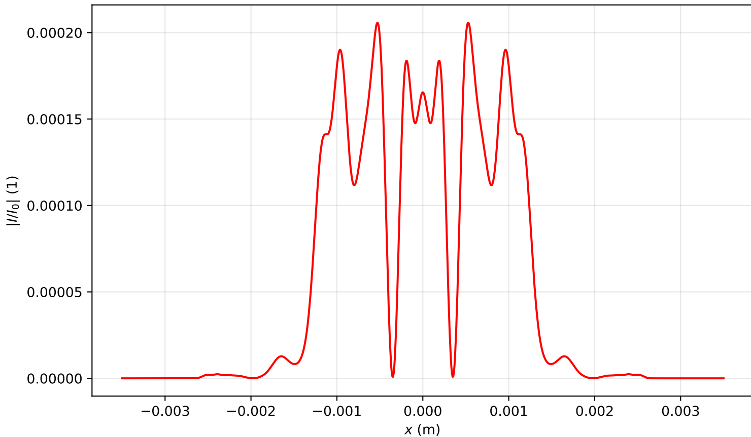
Intensity profile I(x, y = 0, z = 0.955)/I_0 , P_{in}=14.0P_{cr} , artificial time
