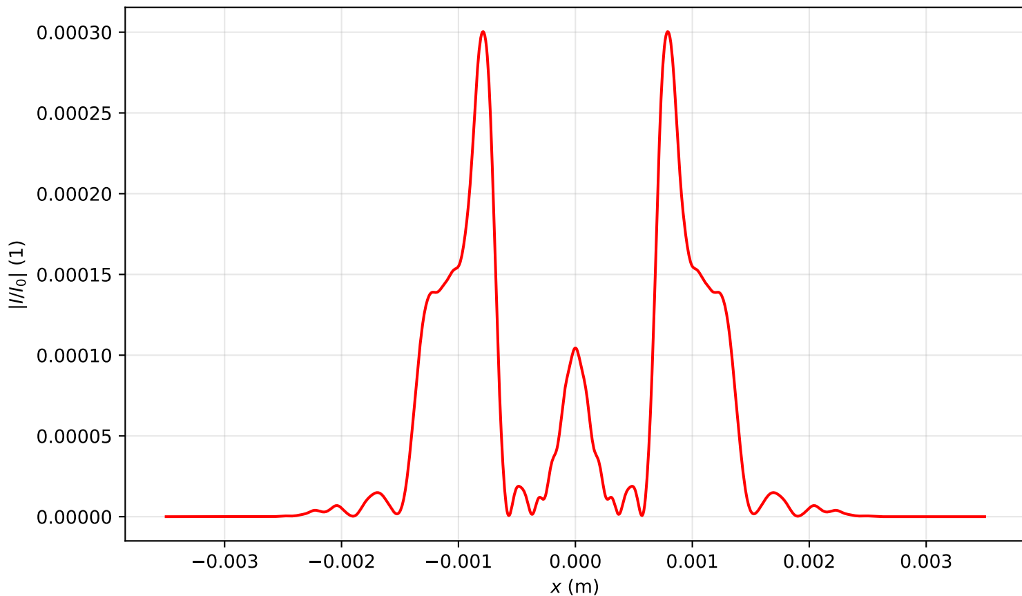
Intensity profile I(x, y = 0, z = 1.194)/I_0 , P_{in}=14.0P_{cr} , artificial time
