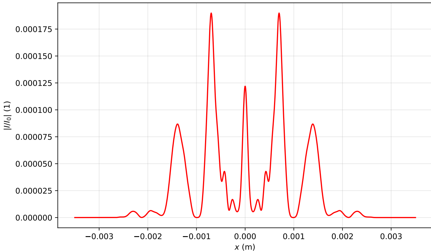
Intensity profile I(x, y = 0, z = 1.274)/I_0 , P_{in}=14.0P_{cr} , artificial time
