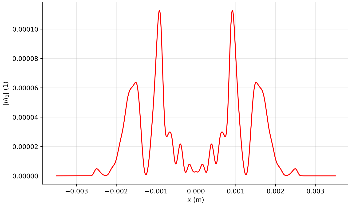
Intensity profile I(x, y = 0, z = 1.592)/I_0 , P_{in}=14.0P_{cr} , artificial time
