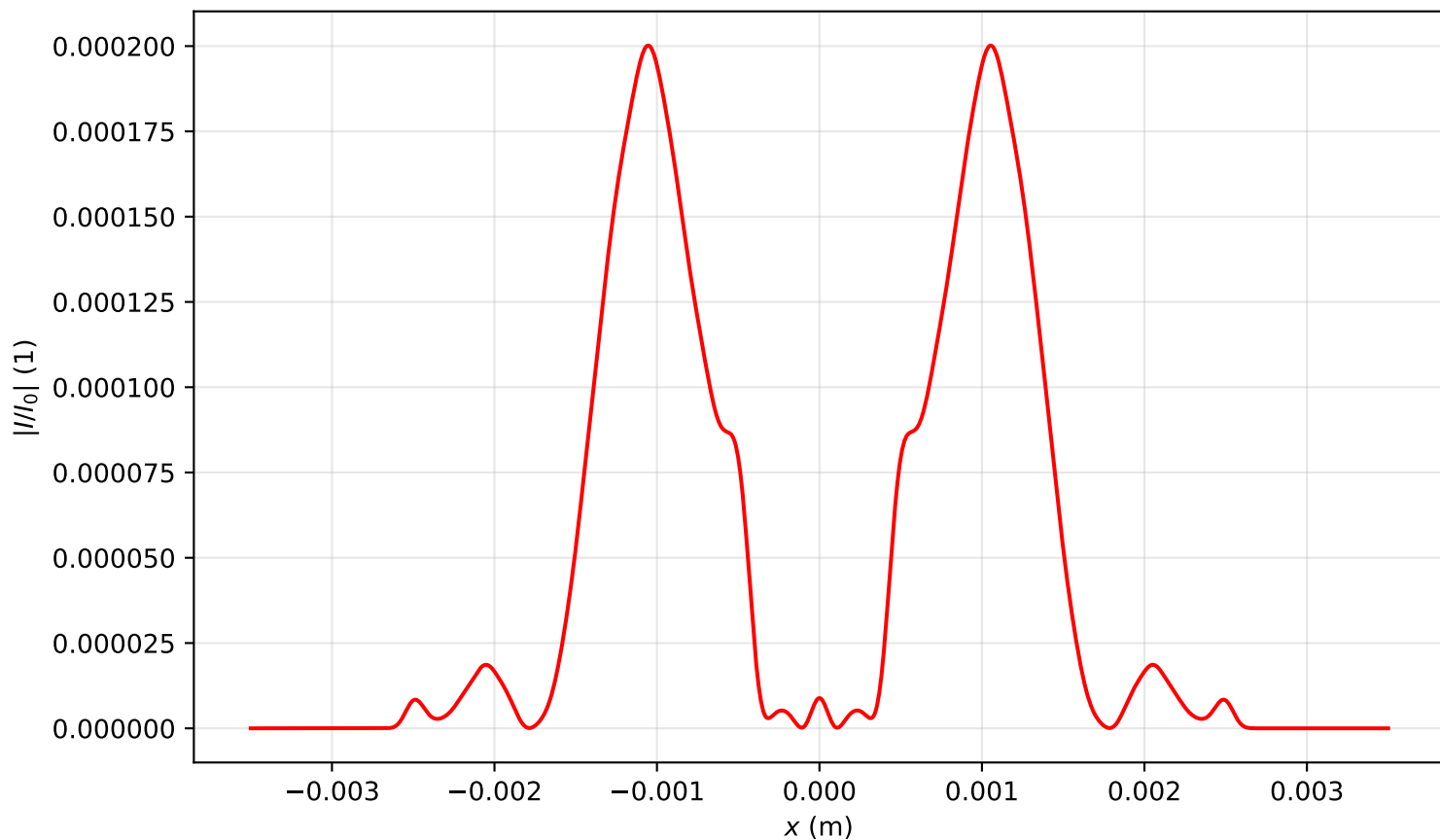
Intensity profile I(x, y = 0, z = 1.990)/I_0 , P_{in}=14.0\text{Pcr} , artificial time
