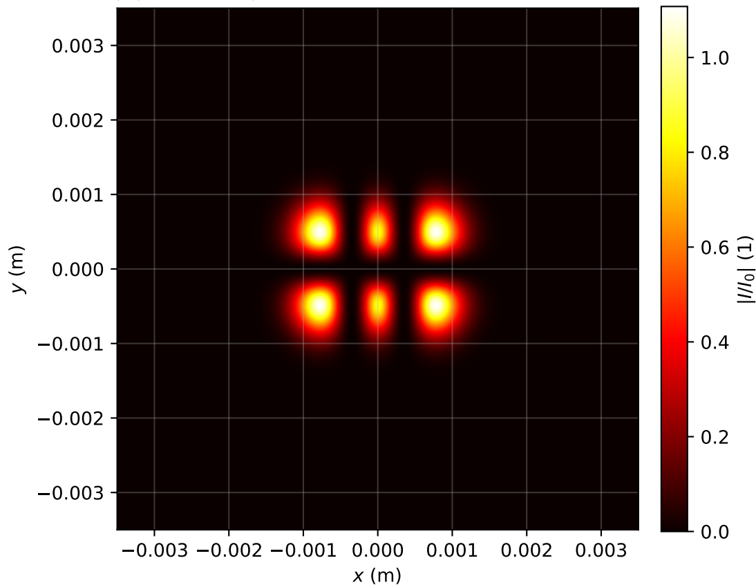
Intensity profile I(x, y, z = 0.080)/I_0 , P_{in}=14.0\text{Pcr} , artificial time
