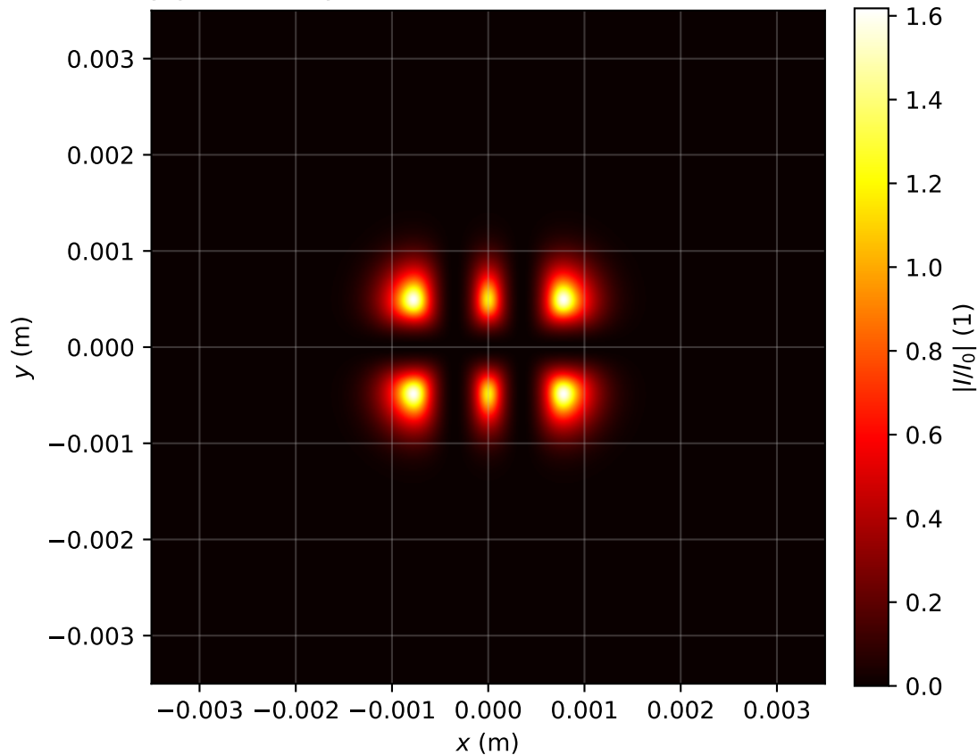
Intensity profile I(x, y, z = 0.159)/I_0 , P_{in}=14.0\text{Pcr} , artificial time
