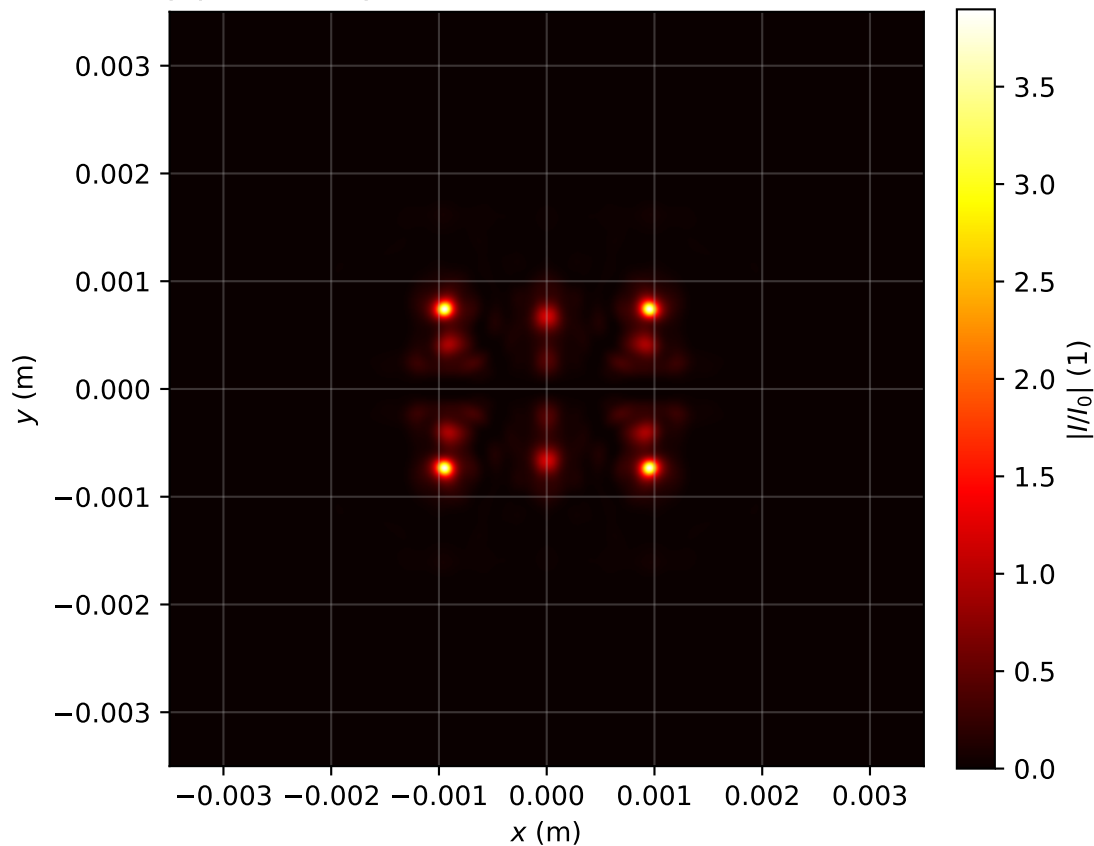
Intensity profile I(x, y, z = 1.115)/I_0 , P_{in}=14.0\text{Pcr} , artificial time
