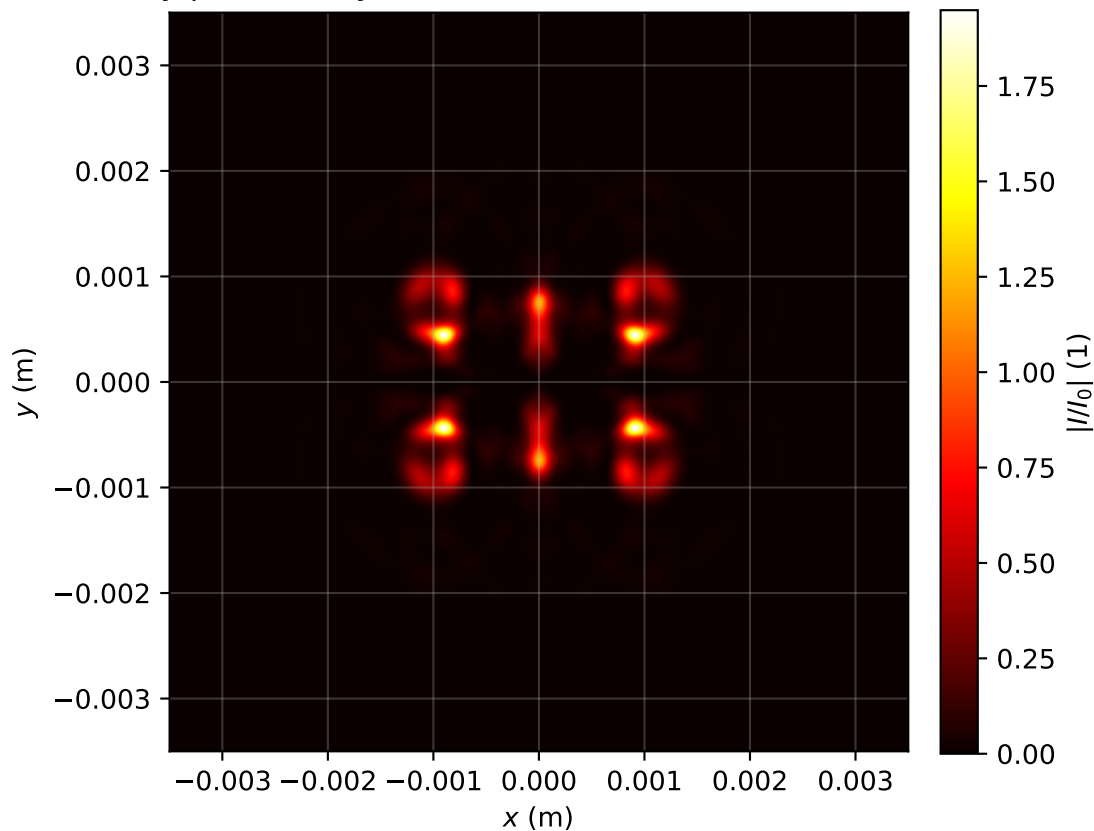
Intensity profile I(x, y, z = 1.274)/I_0 , P_{in}=14.0P_{cr} , artificial time
