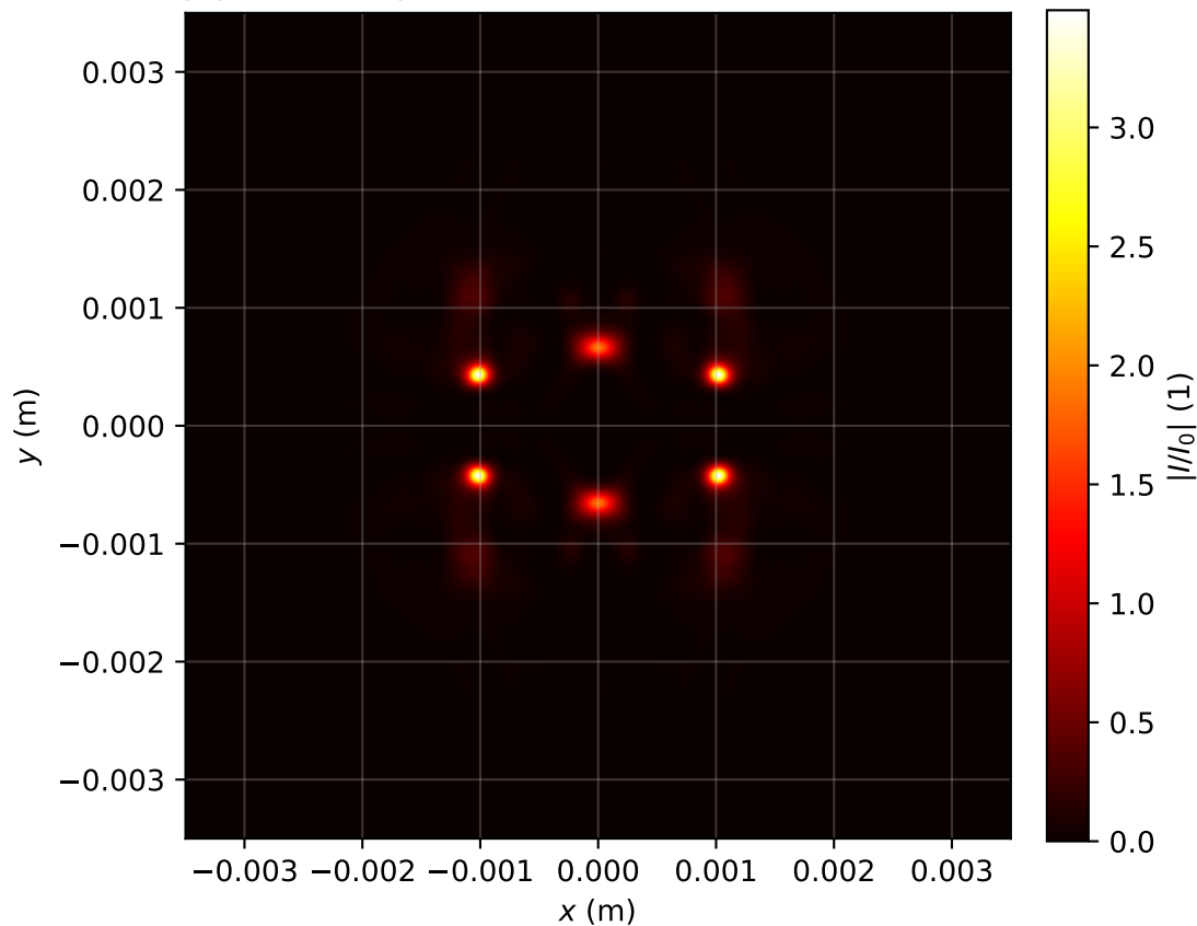
Intensity profile I(x, y, z = 1.672)/I_0 , P_{in}=14.0\text{Pcr} , artificial time
