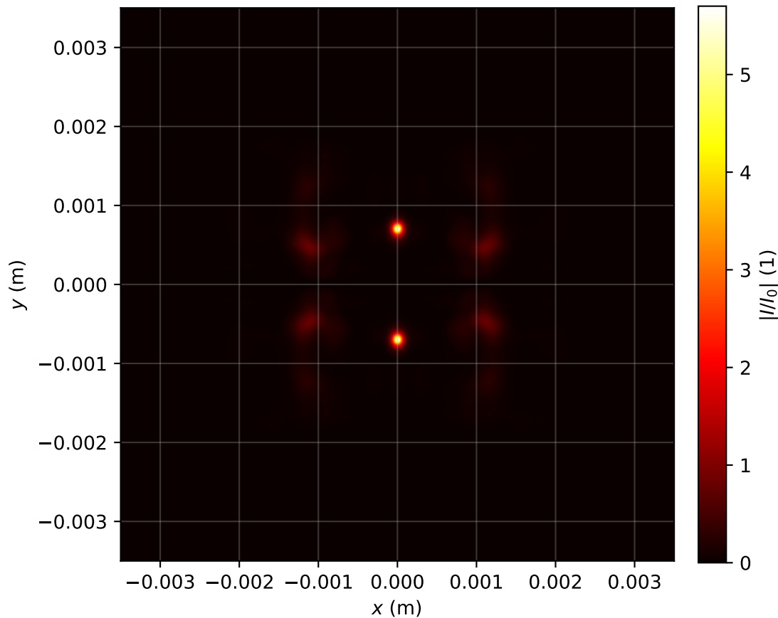
Intensity profile I(x, y, z = 1.831)/I_0 , P_{in}=14.0P_{cr} , artificial time
