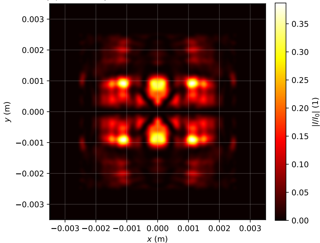
Intensity profile I(x, y, z = 2.388)/I_0 , P_{in}=14.0P_{cr} , artificial time
