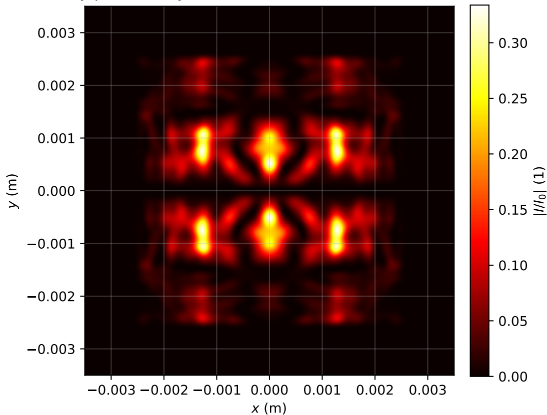
Intensity profile I(x, y, z = 2.627)/I_0 , P_{in}=14.0P_{cr} , artificial time
