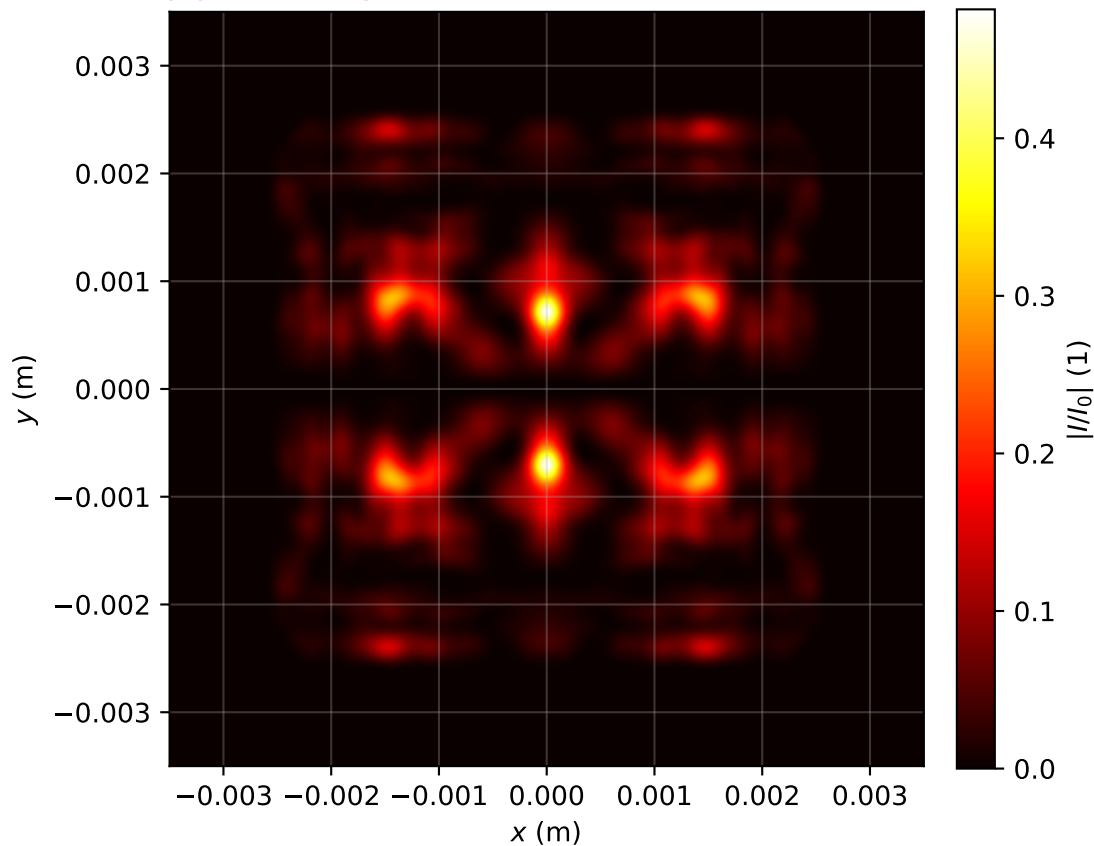
Intensity profile I(x, y, z = 2.866)/I_0 , P_{in}=14.0P_{cr} , artificial time
