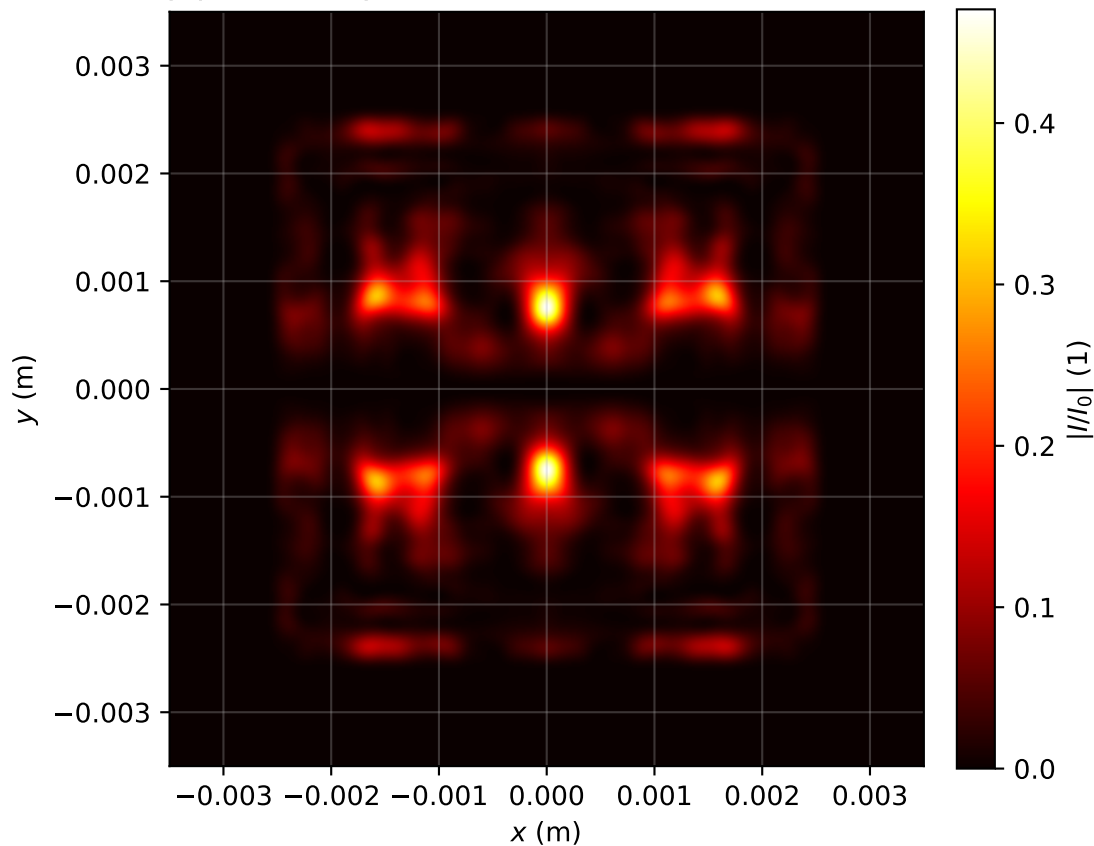
Intensity profile I(x, y, z = 3.025)/I_0 , P_{in}=14.0\text{Pcr} , artificial time
