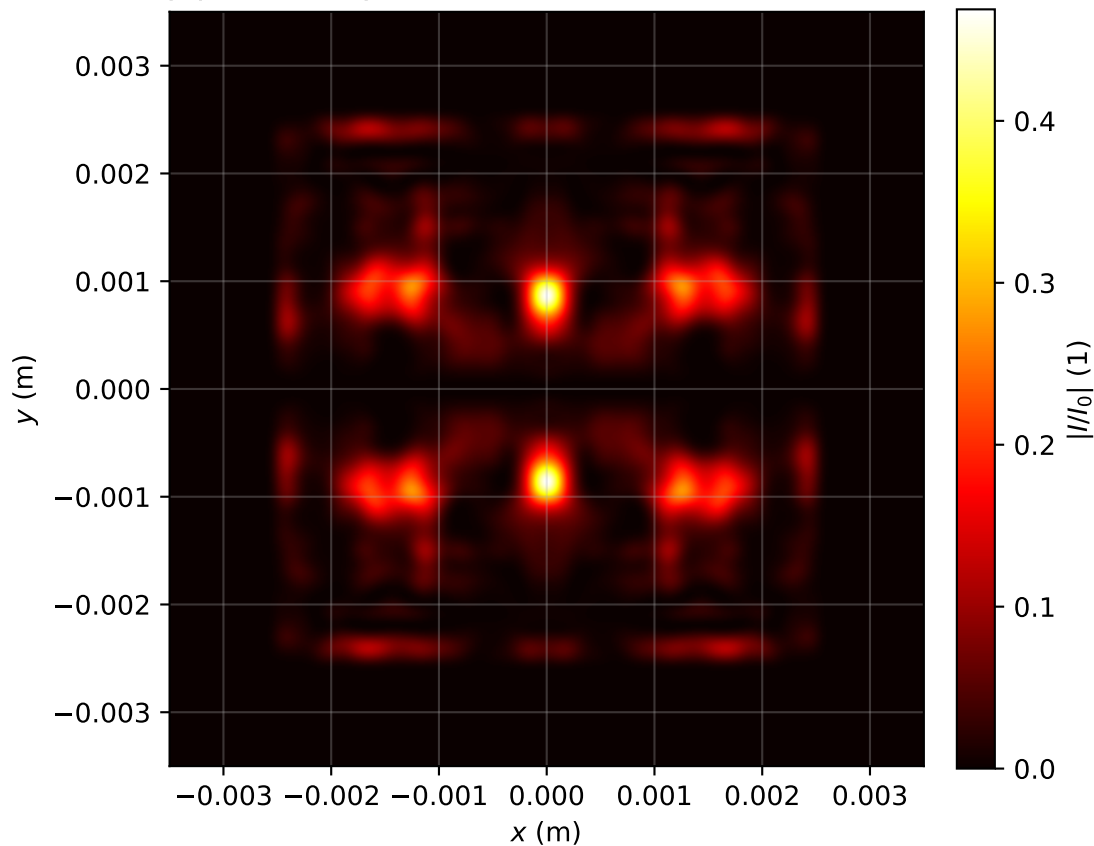
Intensity profile I(x, y, z = 3.184)/I_0 , P_{in}=14.0\text{Pcr} , artificial time
