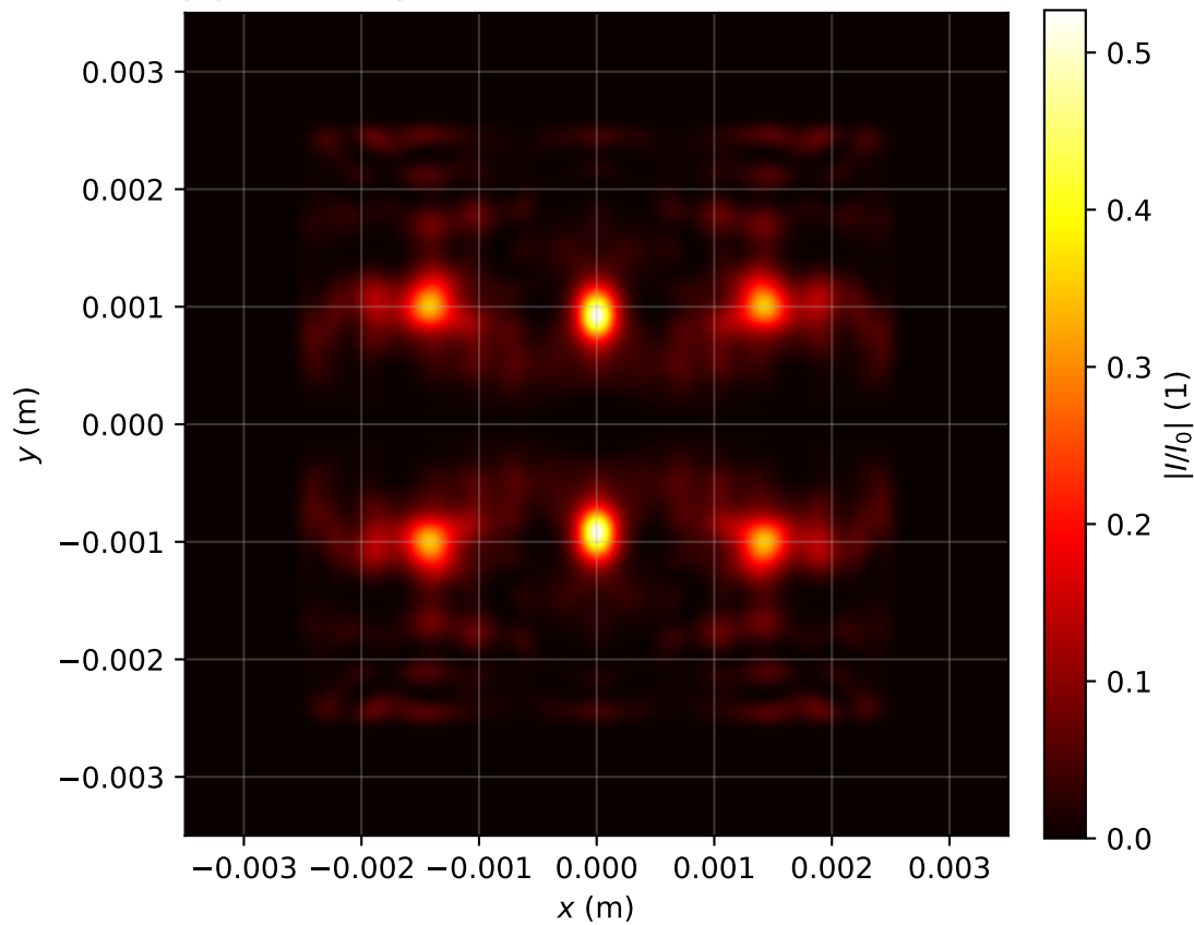
Intensity profile I(x, y, z = 3.423)/I_0 , P_{in}=14.0\text{Pcr} , artificial time
