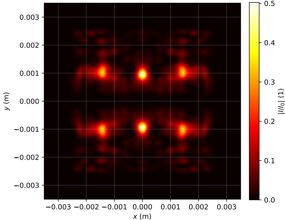
Intensity profile I(x, y, z = 3.503)/I_0 , P_{in}=14.0\text{Pcr} , artificial time
