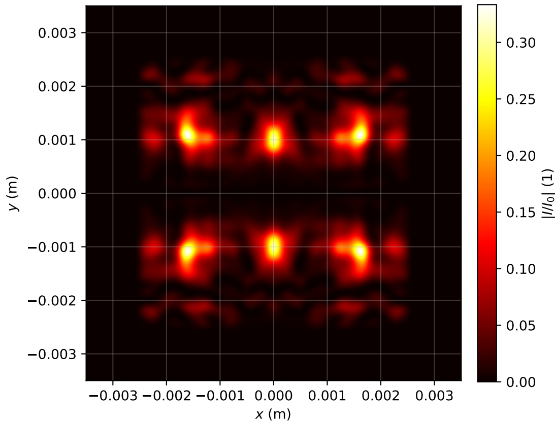
Intensity profile I(x, y, z = 3.901)/I_0 , P_{in}=14.0P_{cr} , artificial time
