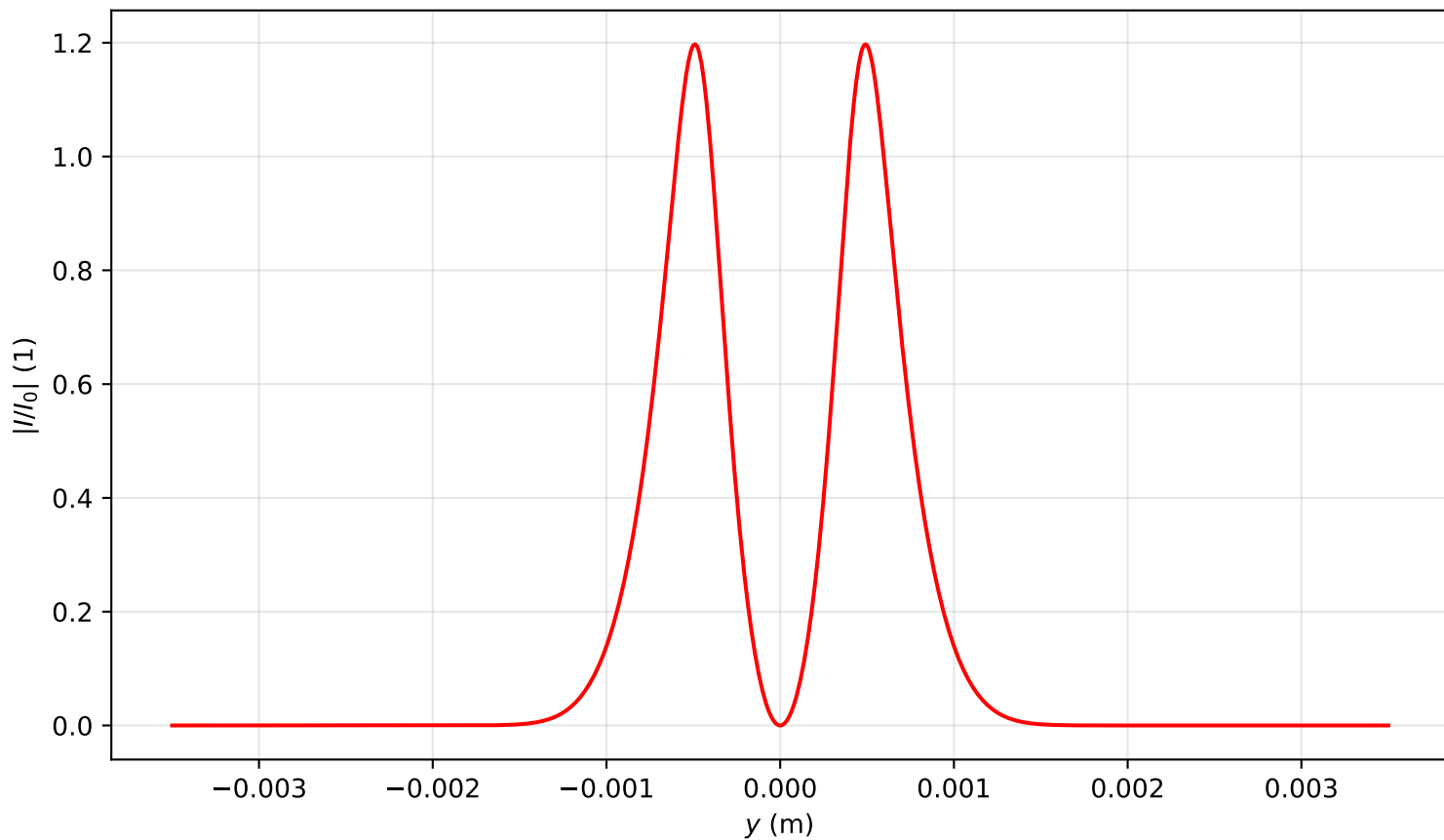
Intensity profile I(x=0, y, z=0.159)/I_0 , P_{in}=14.0P_{cr} , artificial time
