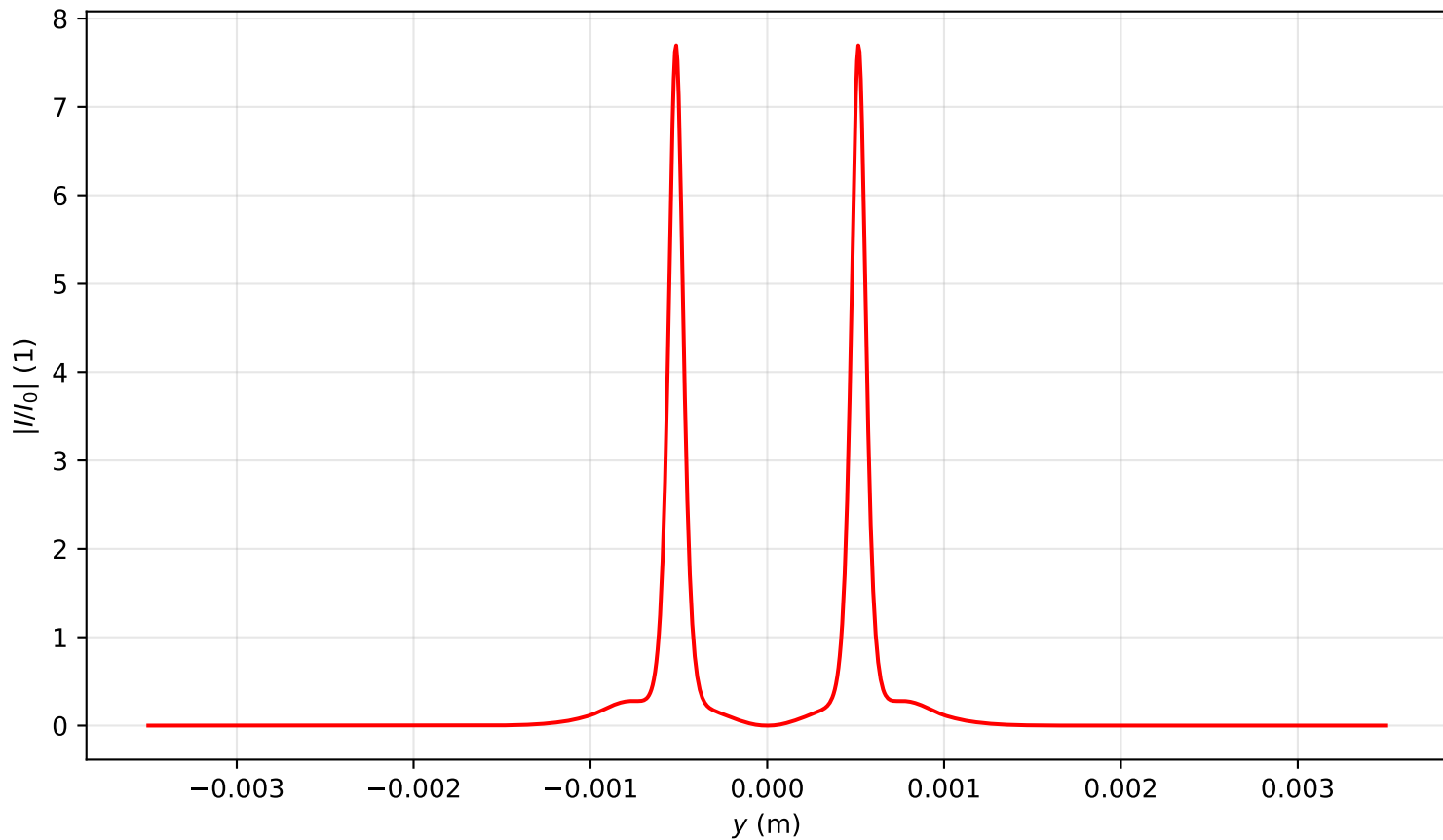
Intensity profile I(x=0, y, z=0.398)/I_0 , P_{in}=14.0P_{cr} , artificial time
