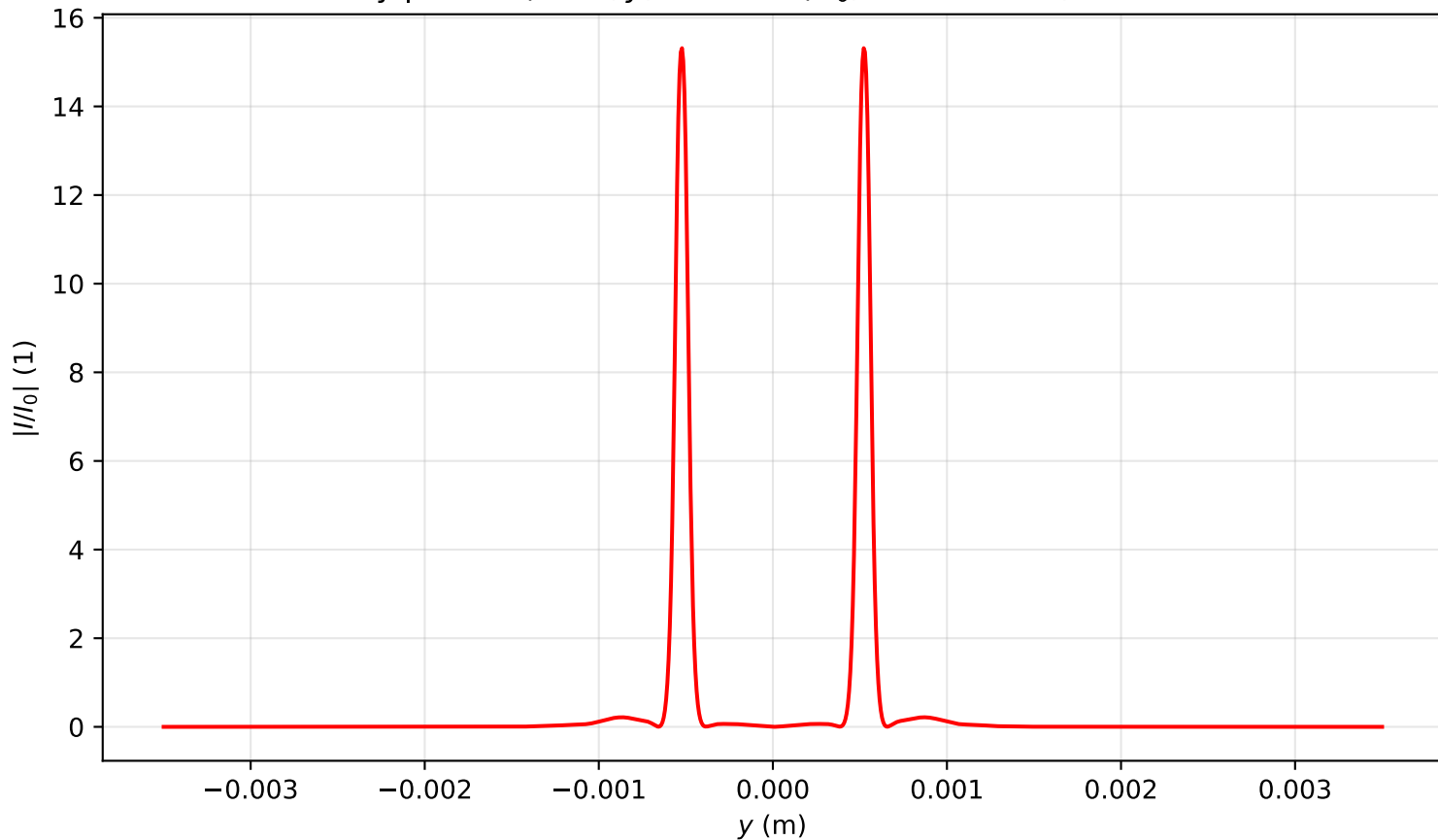
Intensity profile I(x=0, y, z=0.478)/I_0 , Pin=14.0Pcr, artificial time
