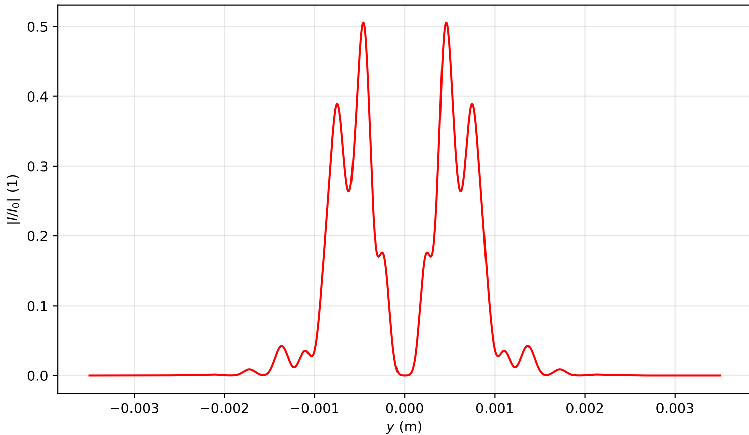
Intensity profile I(x=0, y, z=0.796)/I_0 , P_{in}=14.0P_{cr} , artificial time
